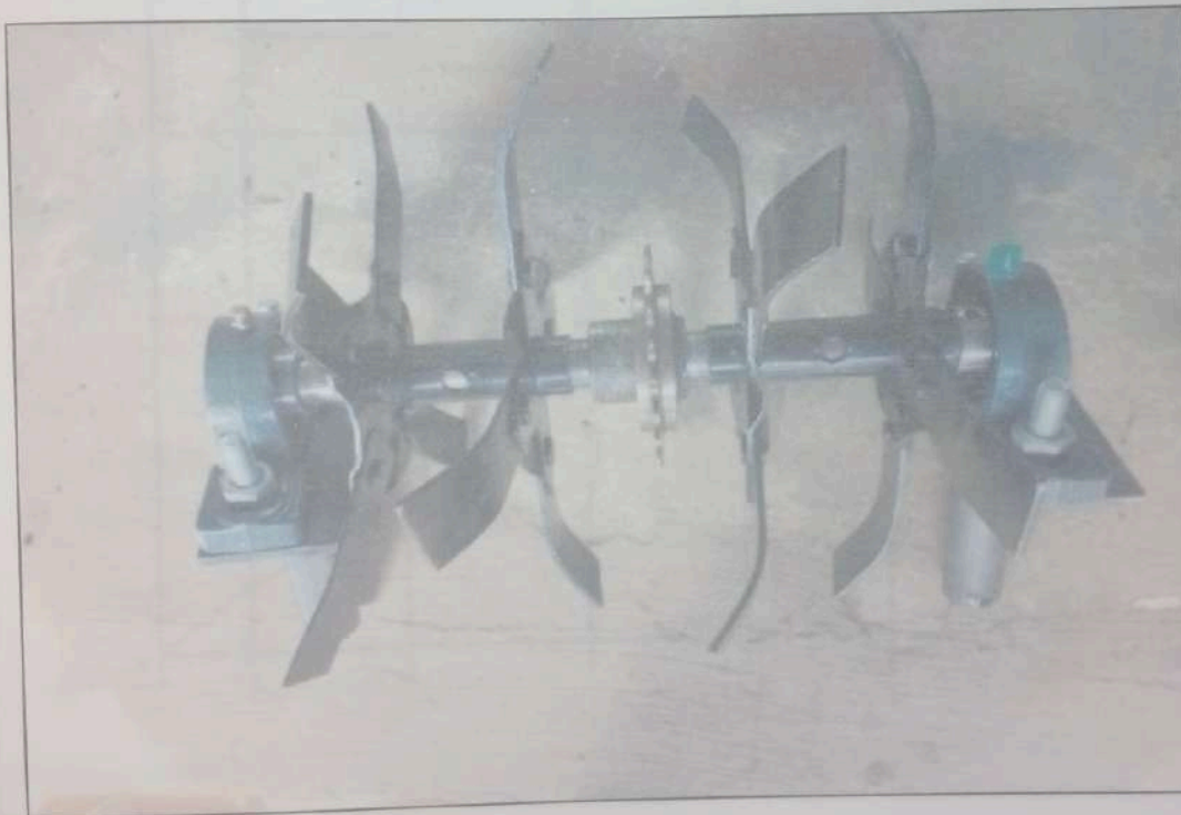
Fig.4.1 Rotor shaft assembly
