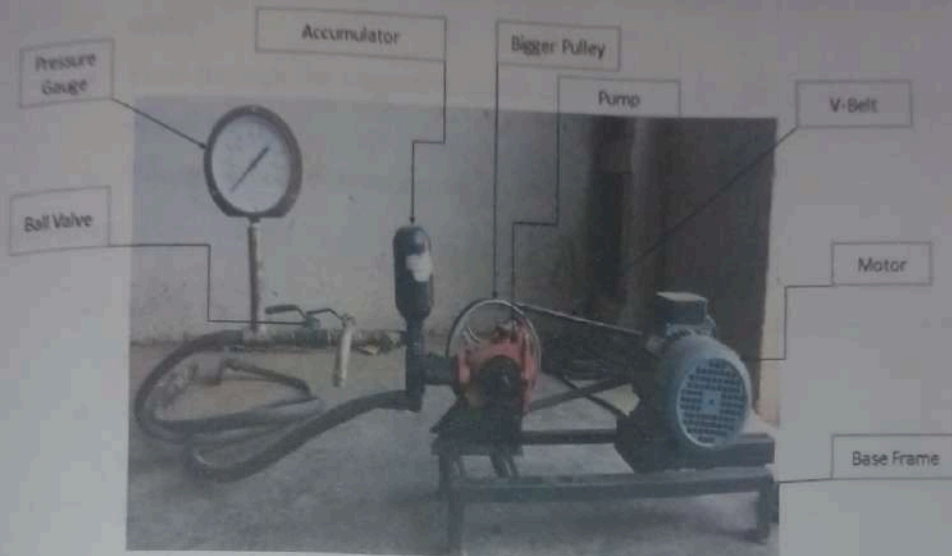
Fig.5.1. Motorized hydraulic valve testing rig
