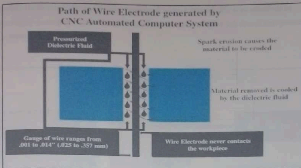
Figure 1.5 Path of wire in WEDM
