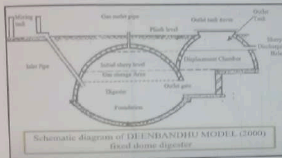
Fig 3.1. Deenbandhu model
