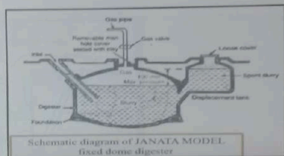
Fig 3.2. Janata model
