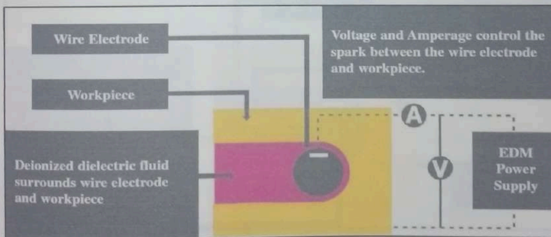
Figure 1.6 Power generation in WEDM
