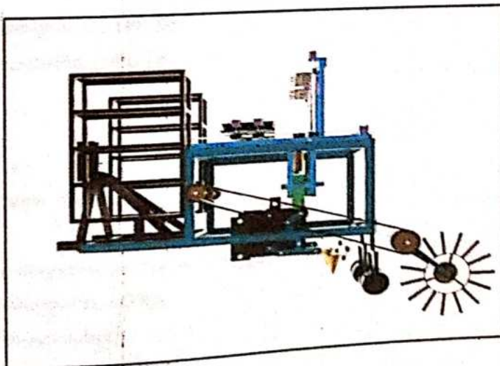
Fig. No. 10. 2 Side View
