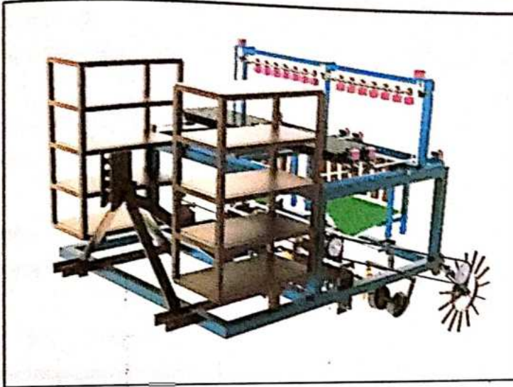
Fig. No. 10. 1 Isometric View
